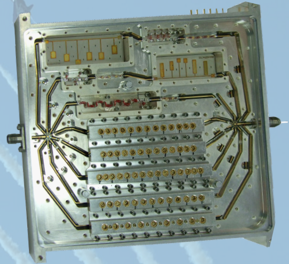
MULTI TECHNOLOGY FILTER BANK
