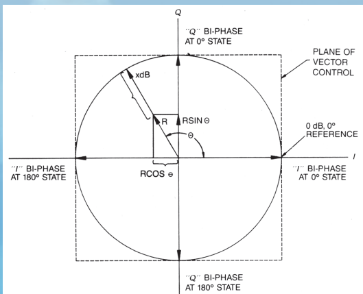
VECTOR MODULATOR
