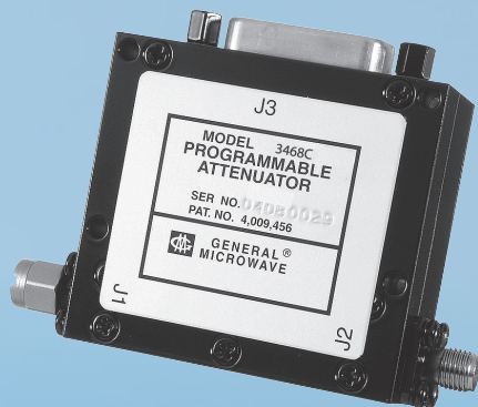
2 to 18 GHz ATTENUATOR
