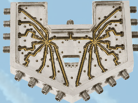
SP16T SWITCH
