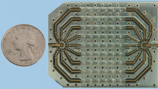
9 CHANNEL FILTER BANK
