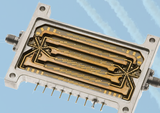
6 CHANNEL FILTER BANK
