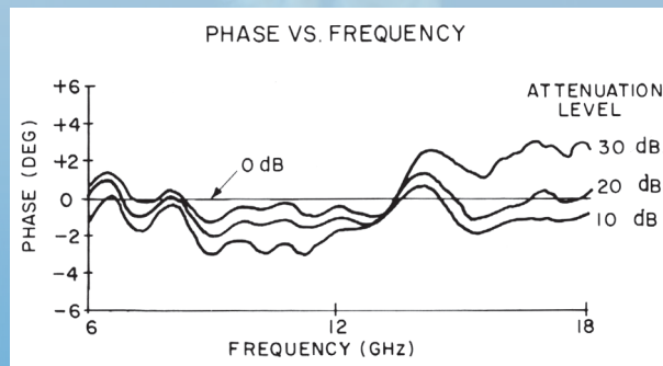
PHASE INVARIANT ATTENUATOR
